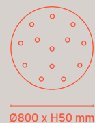
ROUND Ø80 max 13 attacchi / fittings
